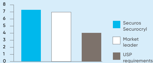
USP <881> Knot-pull tensile 3/0 PGCL suture
